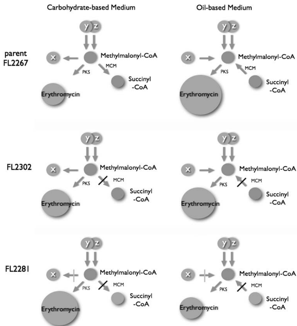
Fig. 3 Metabolic model for erythromycin production by three strains in carbohydrate and oil-based fermentation media. The MCM arrow indicates the reaction catalyzed by MCM whose net flow is in the direction shown in the two different media. MCM , methylmalonyl-CoA mutase; PKS , polyketide synthase. FL2267 , wild-type strain; FL2302 , non-polar mutB knockout strain; FL2281 , polar mutB knockout strain. Circles “y” and “z” represent proposed metabolites that flow, via arrows representing unidirectional enzymatic reactions, into the methylmalonyl-CoA pool in both carbohydrate-based and oil-based media. The “x” circle represents a proposed metabolite that flows into the methylmalonyl-CoA pool in the oil-based medium, and flows out of the methylmalonyl-CoA pool in the carbohydrate-based medium via a reversible enzymatic reaction represented by the arrow . Black bars drawn through arrows represent genetic blocks due directly to the mutation in mutB ; gray bars are metabolic blocks due to the polar effects of the mutB knockout in strain FL2281 . The erythromycin circles are drawn to scale based on relative experimental production levels (Fig. 2b). The arrow to erythromycin represents the multistep biosynthetic reactions required for erythromycin production including the polyketide synthase reactions. The sizes of the circles for other metabolites are not meant to reflect their pool sizes
