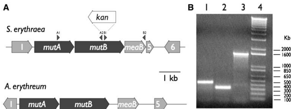
Fig. 1 a Map of the S. erythraea mutAB region (top); A. erythreum mutAB region (bottom); drawn to scale. The DNA sequence for the mutAB region of S. erythraea was submitted previously by the Flores laboratory (accession number AY117133). Additional DNA sequence data were added to both ends of this cluster to expand the figure from 5,894 to 8,204 bp (accession numbers DQ289499 and DQ289500). A1, A2, B1, and B2 triangles indicate primer binding regions as described (Materials and methods). The genes labeled 1, 5, and 6 are referred to in the text as SeORF1 , SeORF5 , and SeORF6 , respectively. The arrow labeled kan represents the kanamycin-resistance gene from pUC4K inserted into the mutB gene of S. erythraea to create the polar knockout strain FL2281 (Materials and methods). New DNA sequence information for the A. erythreum mutAB region in this figure (on both ends of the
